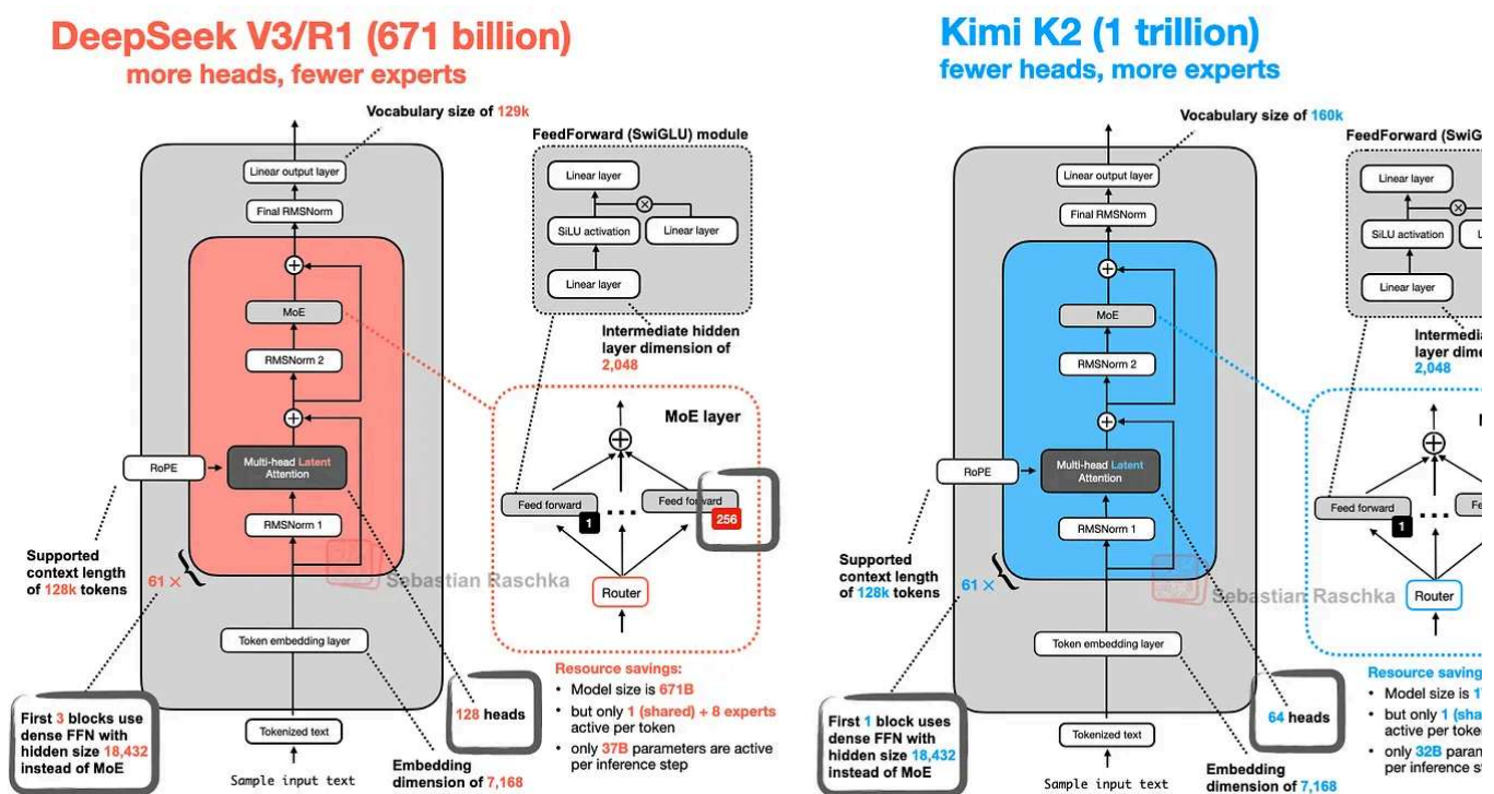
Figure 25.1: An architecture comparison between DeepSeek V3 and Kimi K2.
